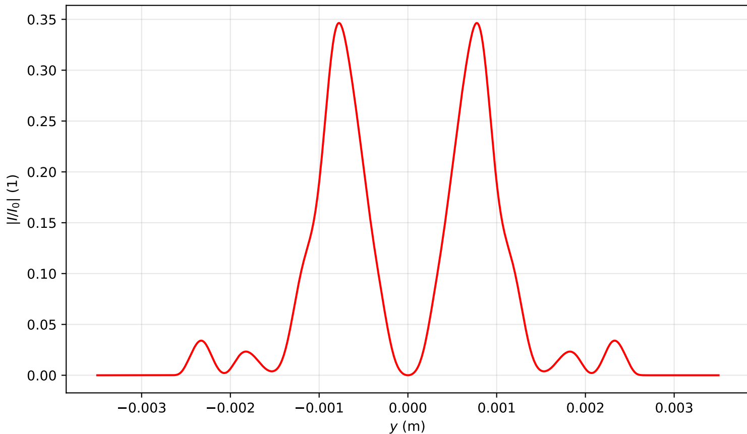
Intensity profile I(x=0, y, z=3.344)/I_0 , P_{in}=6.0P_{cr} , artificial time
